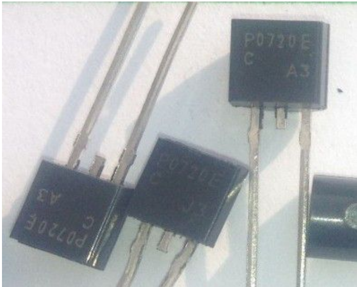
P0720ECL(Marking:P0720EC)
